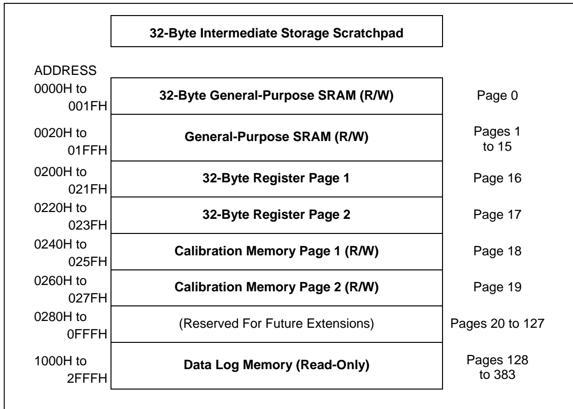
Figure 5. DS1923 MEMORY MAP
